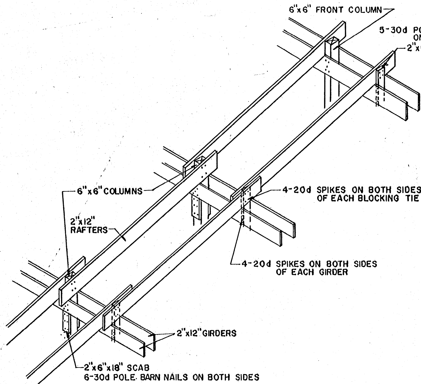
RAFTER DETAIL NOTE ANCHORAGE
