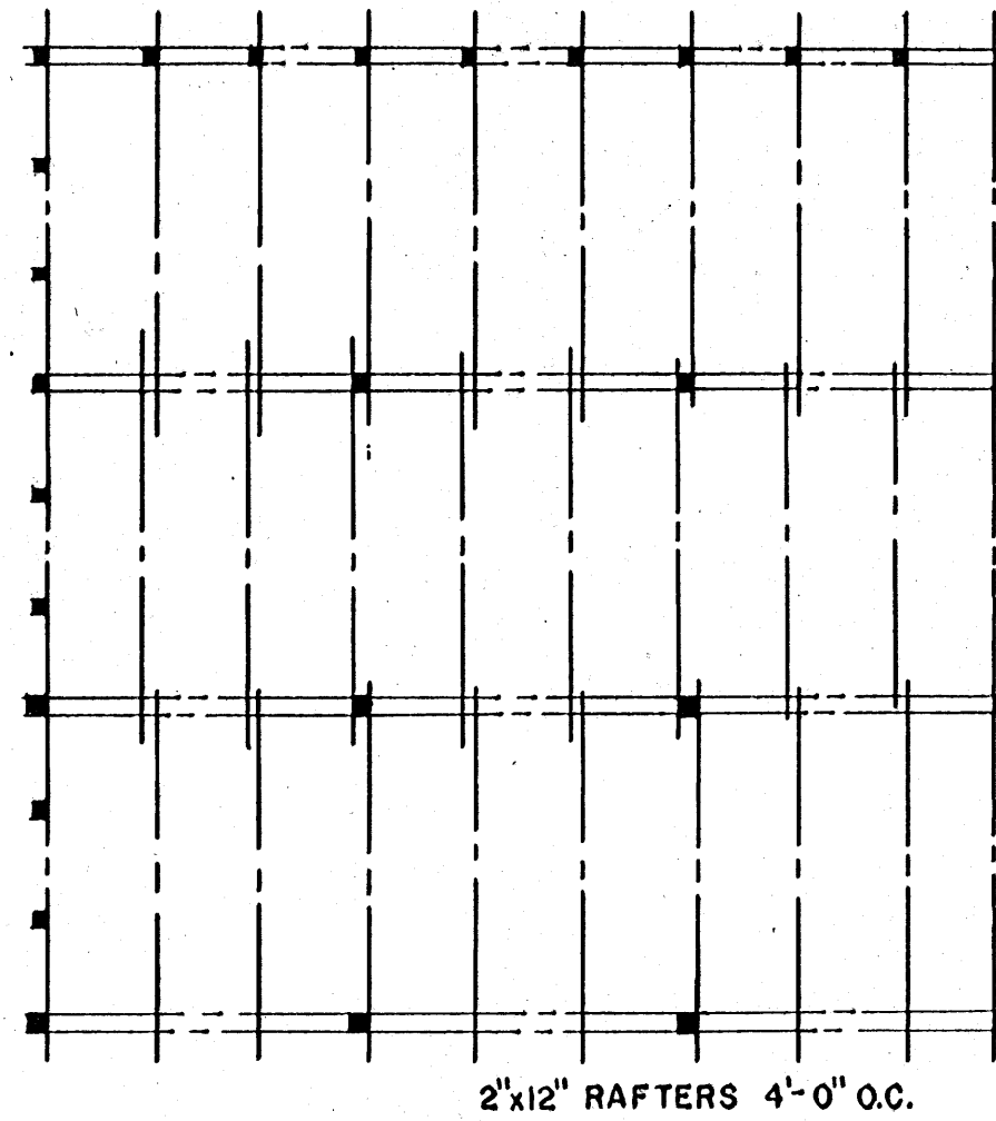
RAFTER LAYOUT
