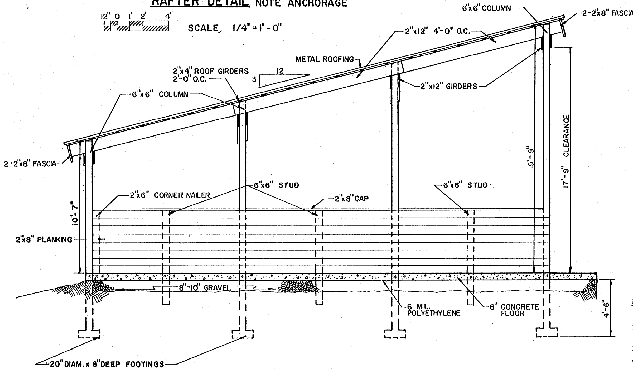
CROSS SECTION
