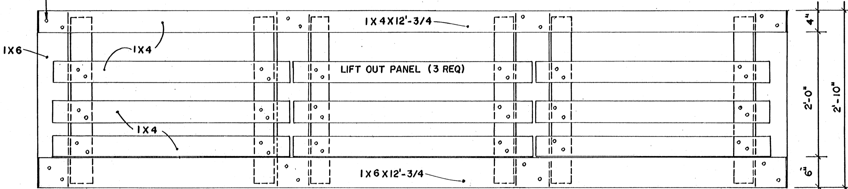
ELEVATION VIEW
