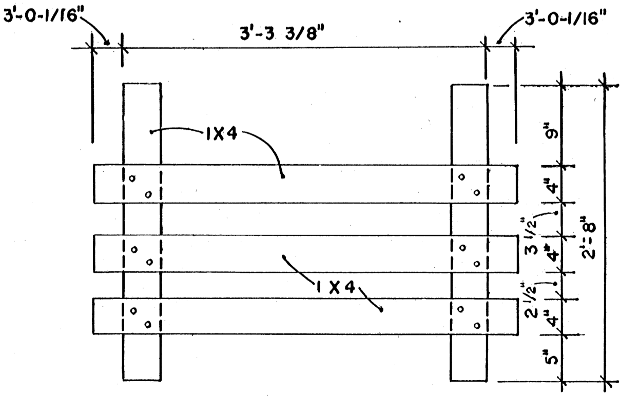
LIFT OUT PANEL DETAILS
