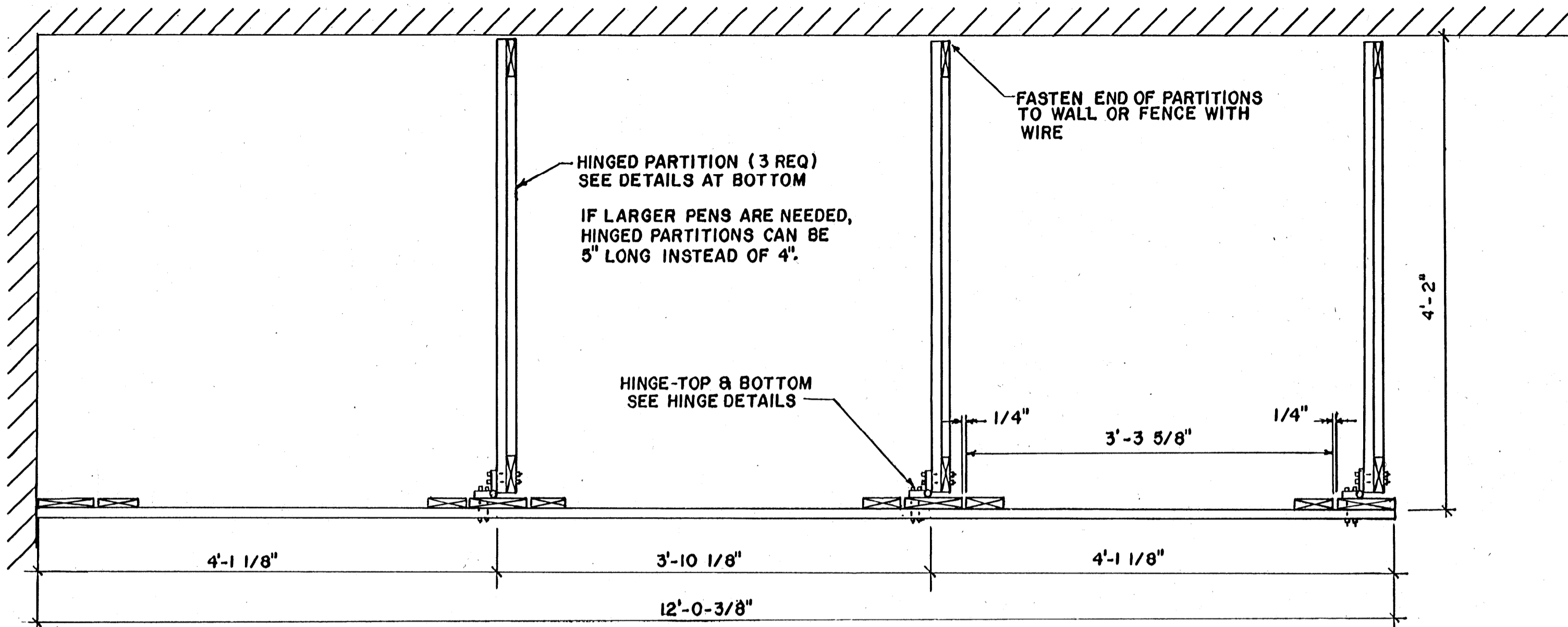
PLAN VIEW
