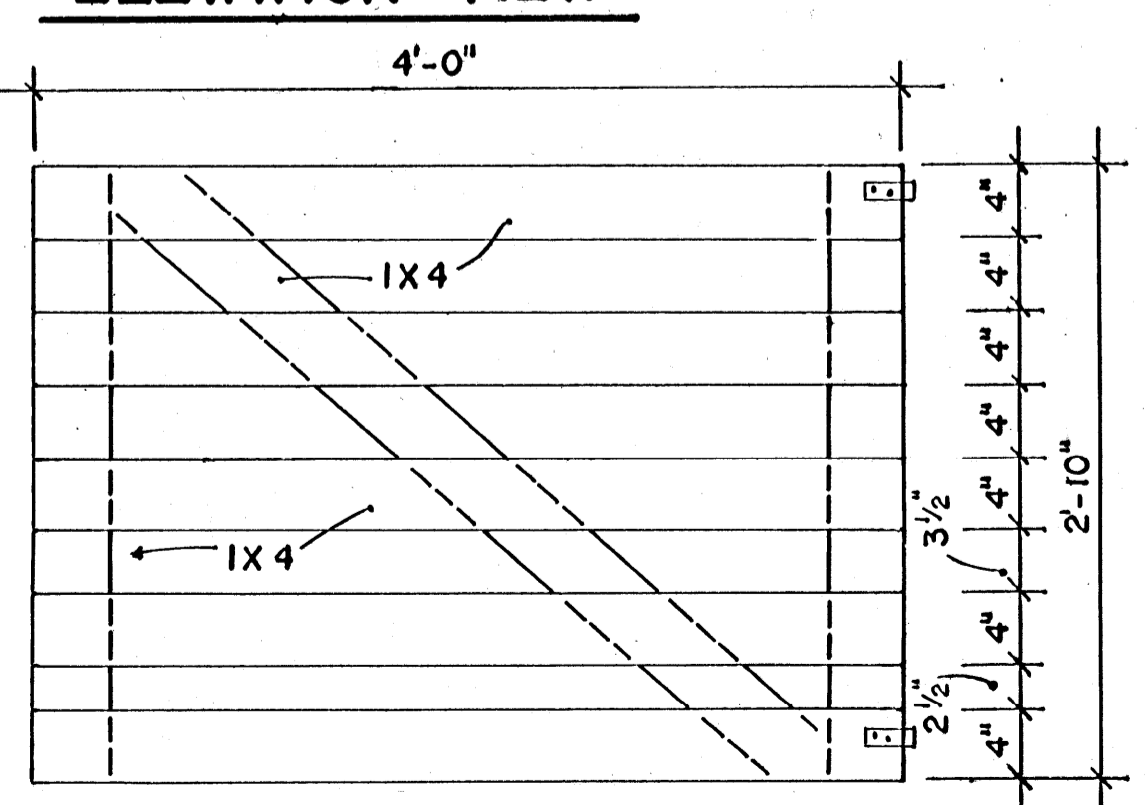
PARTITION DETAILS
