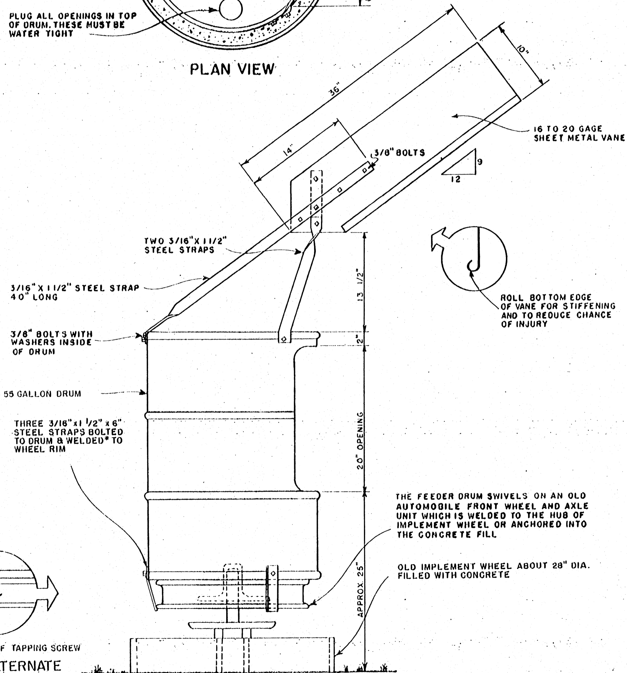
SIDE ELEVATION
